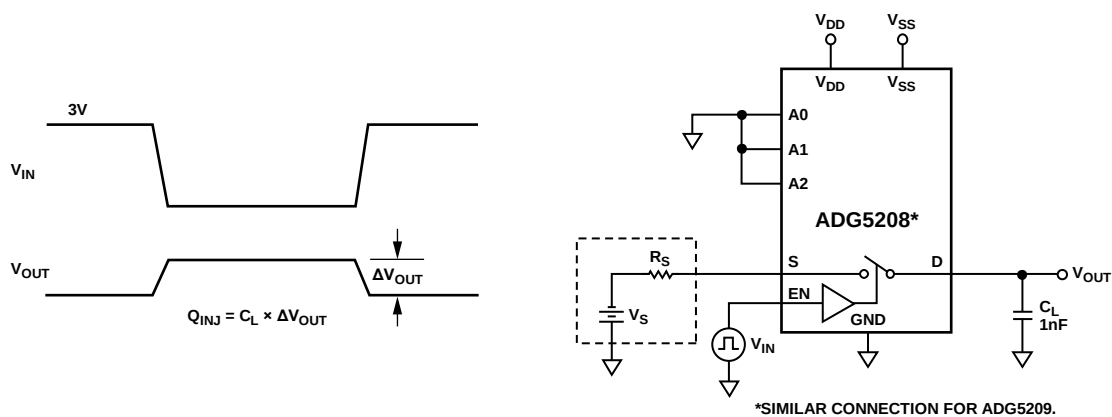
Figure 36. Charge Injection
