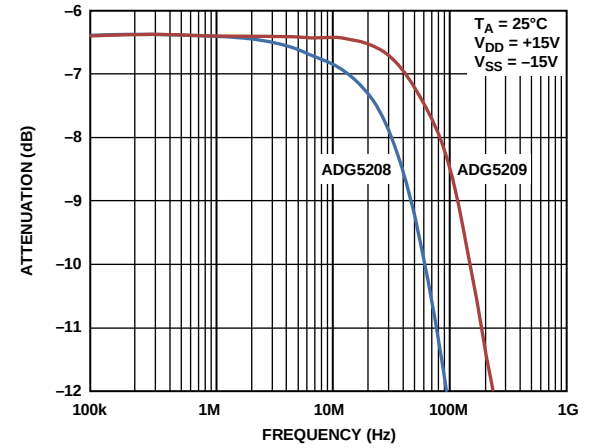
Figure 22. Bandwidth
