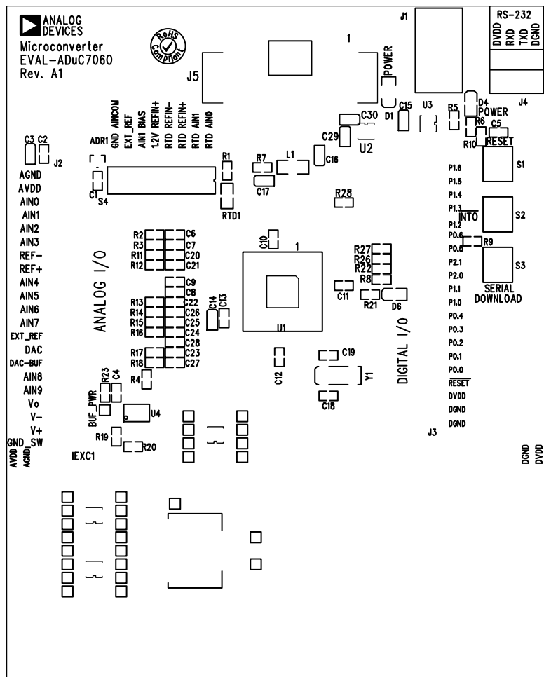
Figure 4. Evaluation Board Silkscreen
