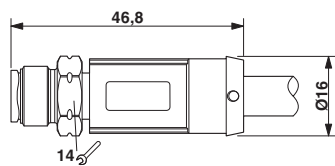
Dimensioned drawing
