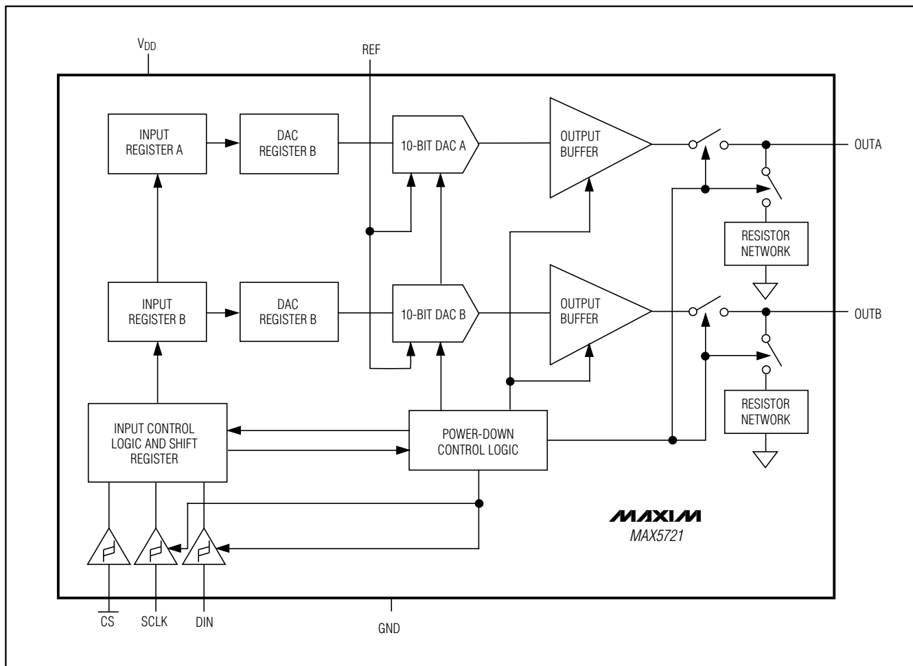
Functional Diagram
