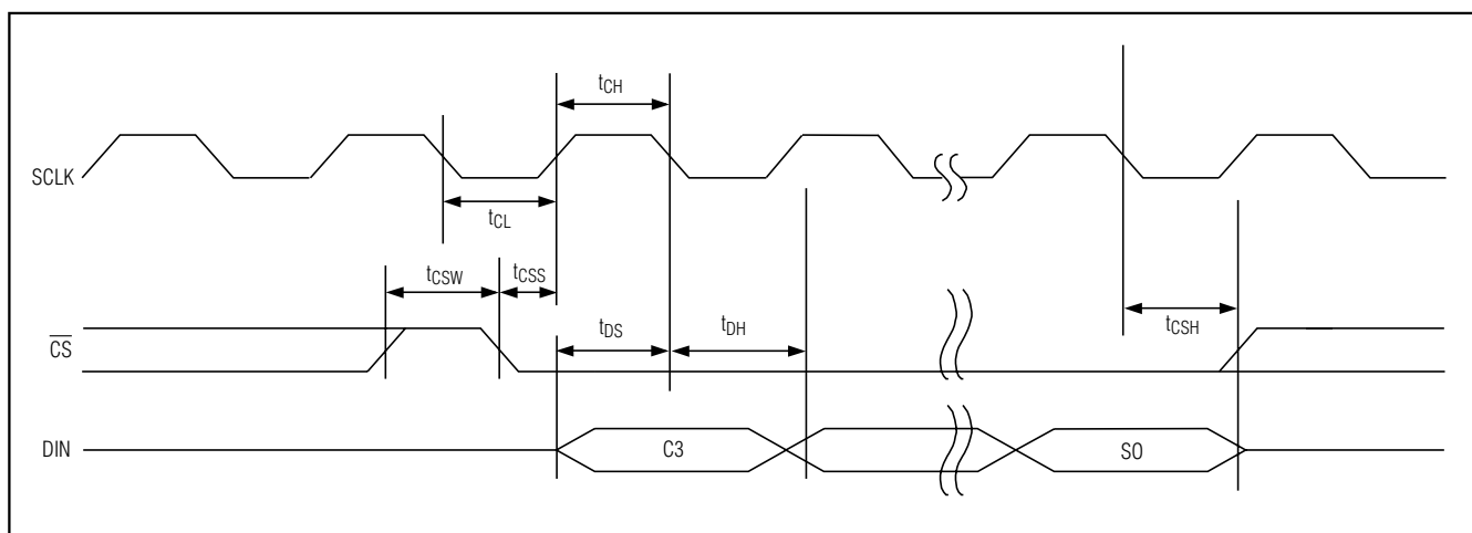
Figure 2. Timing Diagram
