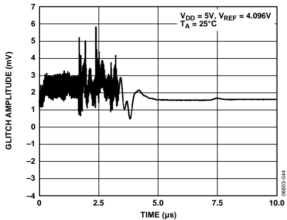
Figure 33. DAC-to-DAC Crosstalk
