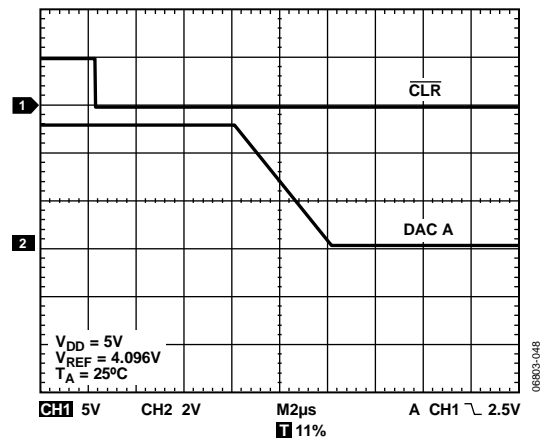
Figure 37. Hardware \overline{CLR}
