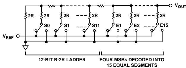
Figure 46. DAC Ladder Structure
