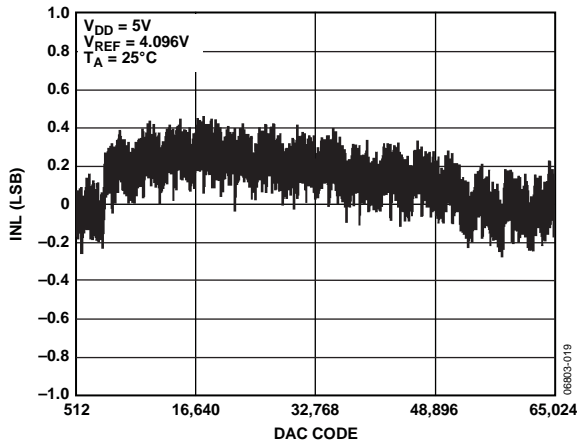
Figure 8. AD5064/AD5064-1 INL
