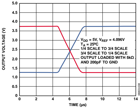
Figure 27. Settling Time
