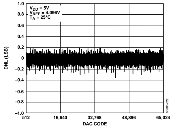
Figure 11. AD5064/AD5064-1 DNL
