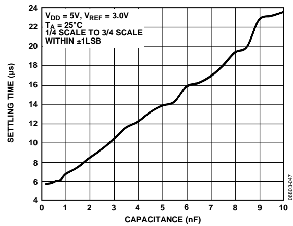
Figure 36. Settling Time vs. Capacitive Load
