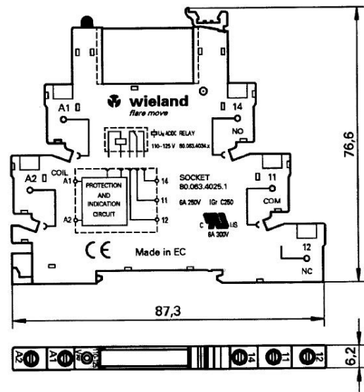
Dimensional diagram
