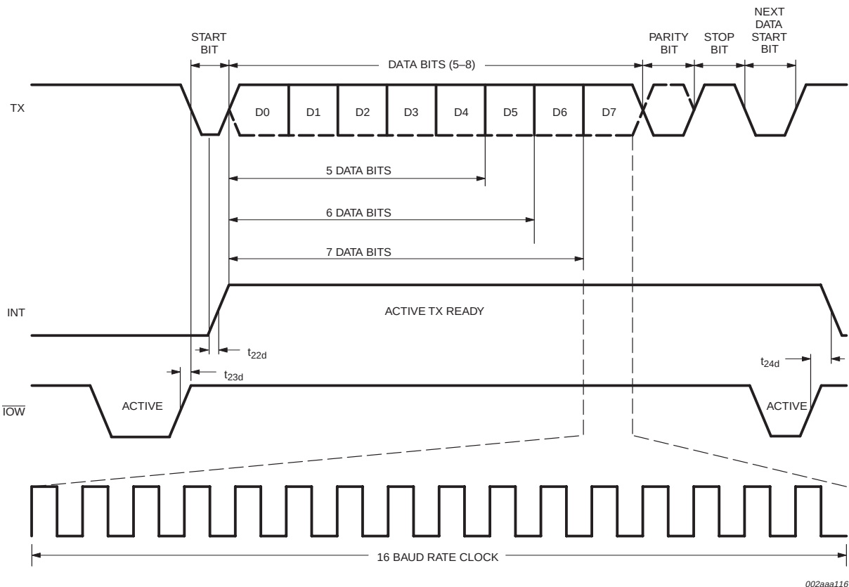
Fig 21. Transmit timing.
