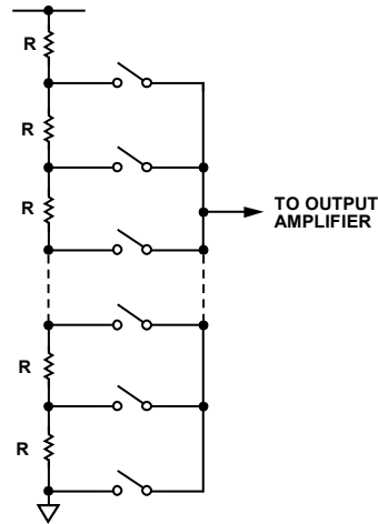
Figure 53. Resistor String
