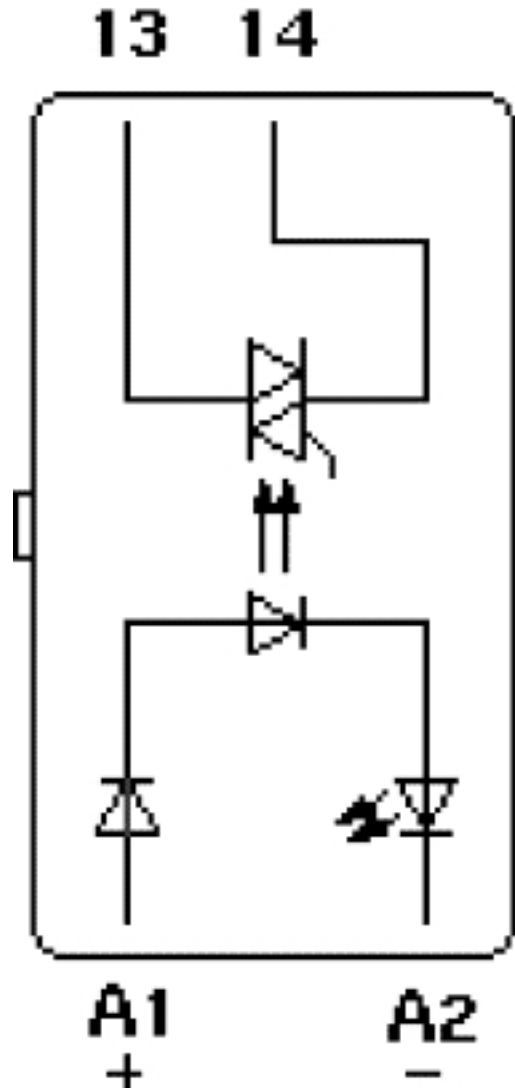
Circuit diagram
