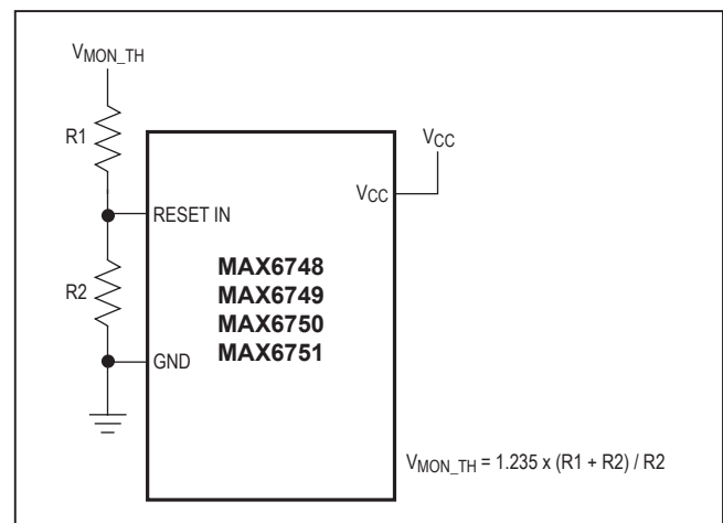
Figure 2. Calculating the Monitored Threshold Voltage ( V_{MON\_TH} )
