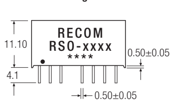
8 PIN SIP Package
