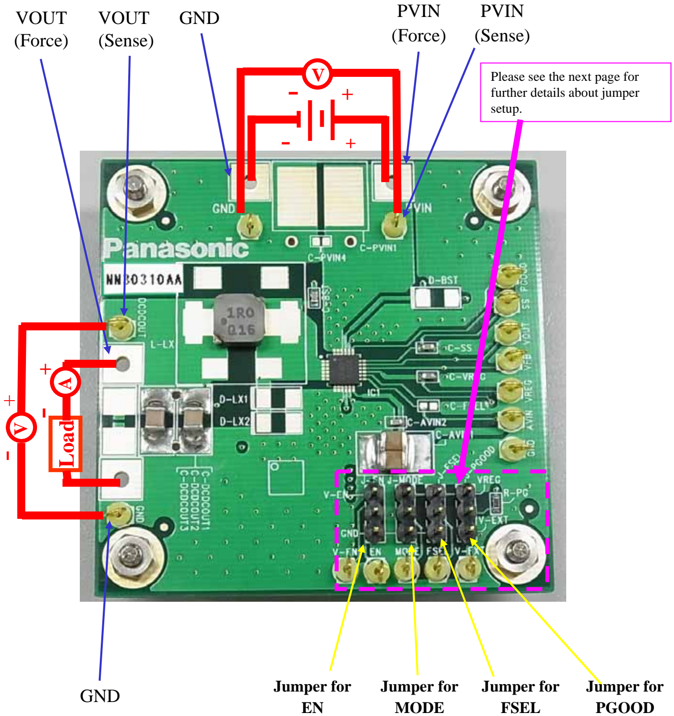
Figure 2. Appearance of Evaluation Board
