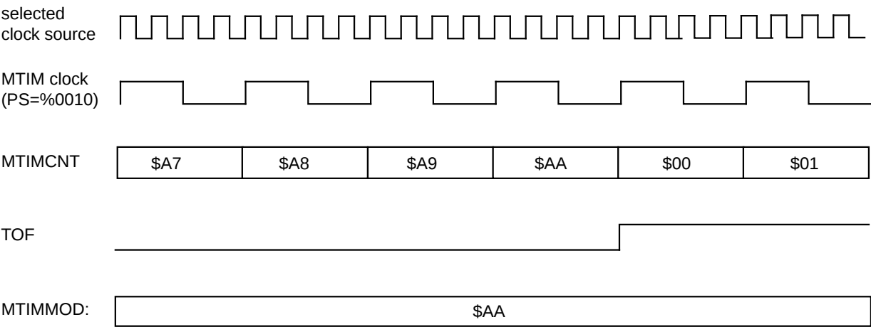
Figure 11-7. MTIM Counter Overflow Example
