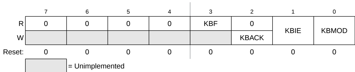
Figure 7-3. KBI Status and Control Register (KBISC)
