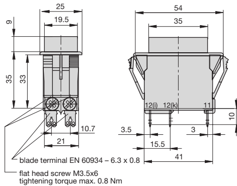
3120-F 3.3 collar height 9 mm
