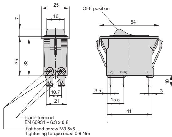
3120-F 3.3 collar height 9 mm
