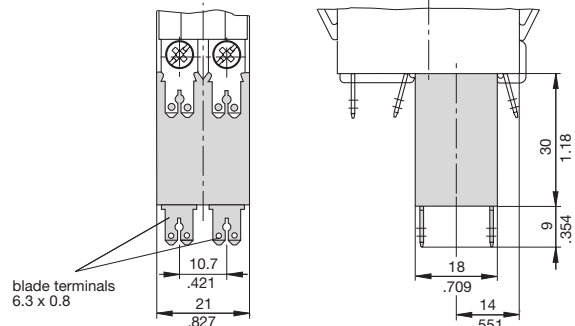
Dimensional drawings of the standard version of 3120-N
