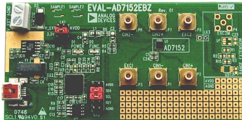
Figure 1. AD7152 Evaluation Board
