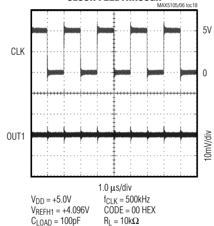
CLOCK FEEDTHROUGH
