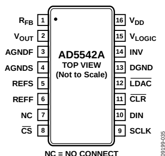
Figure 6. AD5542A 16-Lead TSSOP Pin Configuration
