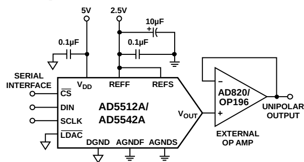
Figure 31. Unipolar Output
