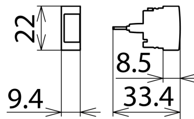
Dimension drawing DRL PD
