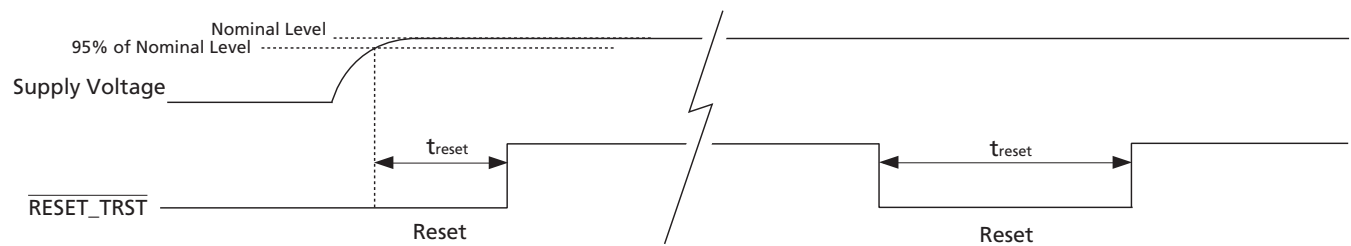
Figure 4-41: Reset Pulse
