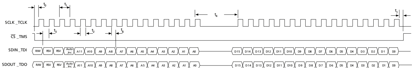
Figure 4-36: Write Mode
