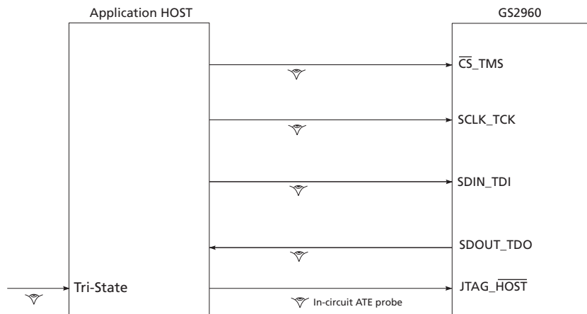
Figure 4-40: System JTAG
