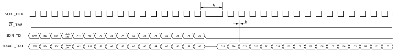
Figure 4-37: Read Mode
