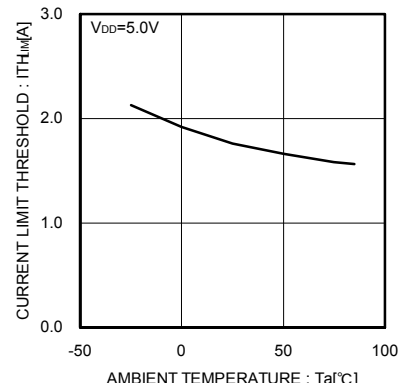
Fig.20 Over current threshold
