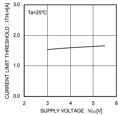
Fig.19 Over current threshold
