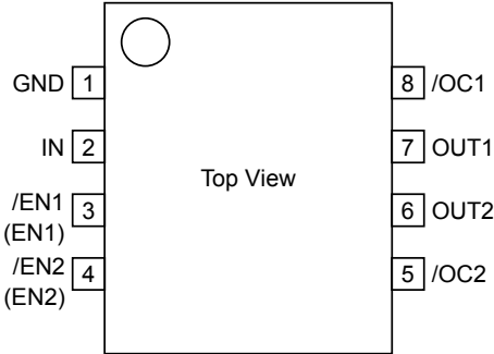
Fig.86 Pin Configuration
