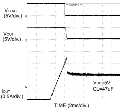
Fig.74 Over current response Ramped load (BD6512F)
