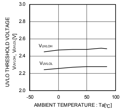
Fig.17 UVLO threshold voltage
