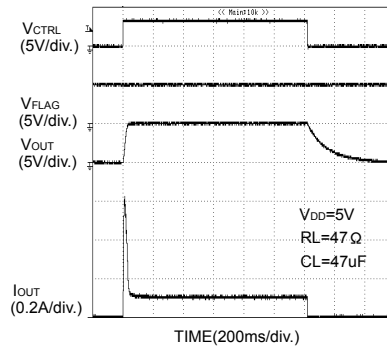
Fig.72 Output rise, fall characteristic (BD6516F)
