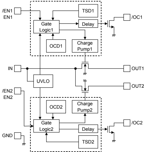
Fig.85 Block diagram
