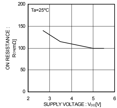
Fig.57 ON resistance
