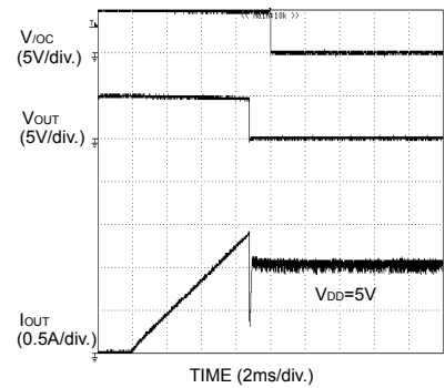
Fig.76 Over current response Ramped load (BD2052AFJ)
