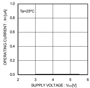
Fig.23 Operating current CTRL Disable
