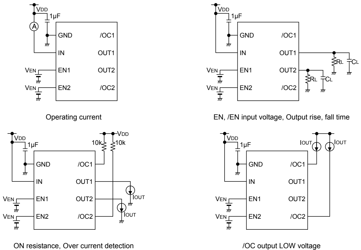
Fig.1 Measurement circuit
