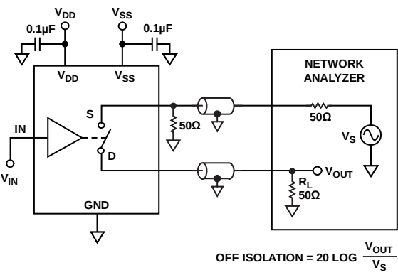
Figure 25. Off Isolation
