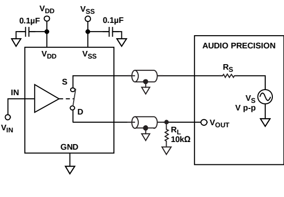
Figure 27. THD + N
