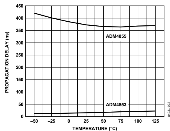
Figure 14. Driver Propagation Delay vs. Temperature
