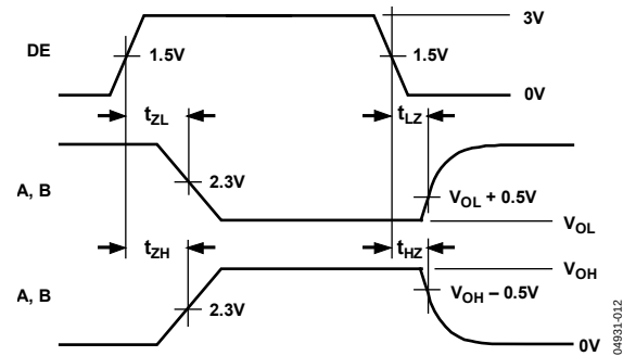
Figure 26. Driver Enable/Disable Timing
