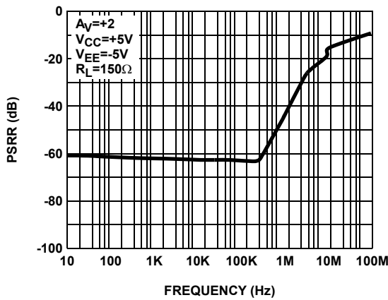
FIGURE 13. PSRR ( V_{EE} )
