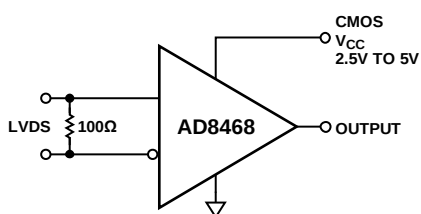
Figure 13. LVDS-to-CMOS Receiver
