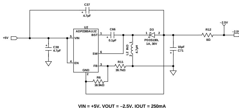
Figure 24. Schematic Page 1
