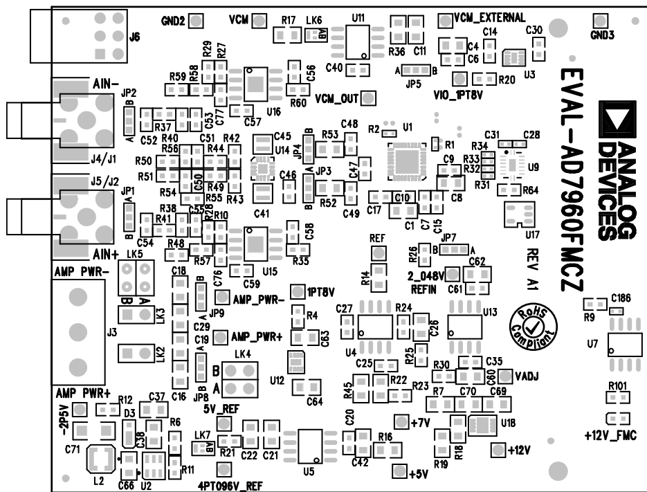
Figure 30. EVAL-AD7960FMCZ Evaluation Board Silkscreen—Top Assembly
