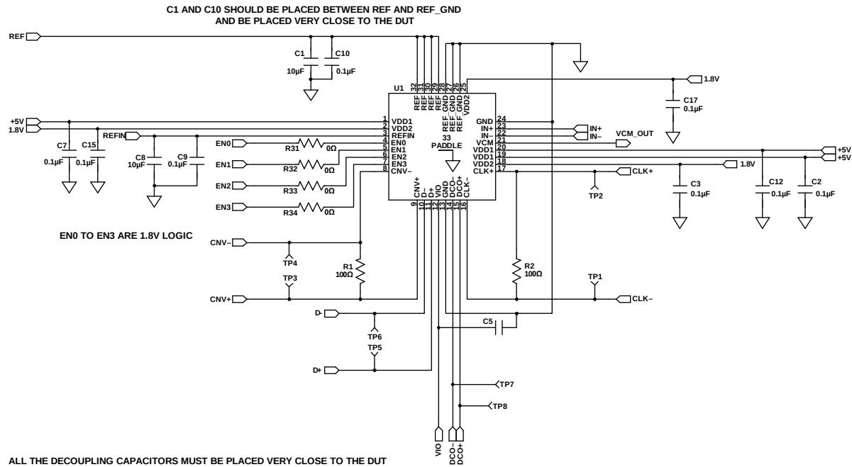
Figure 28. Schematic Page 5
