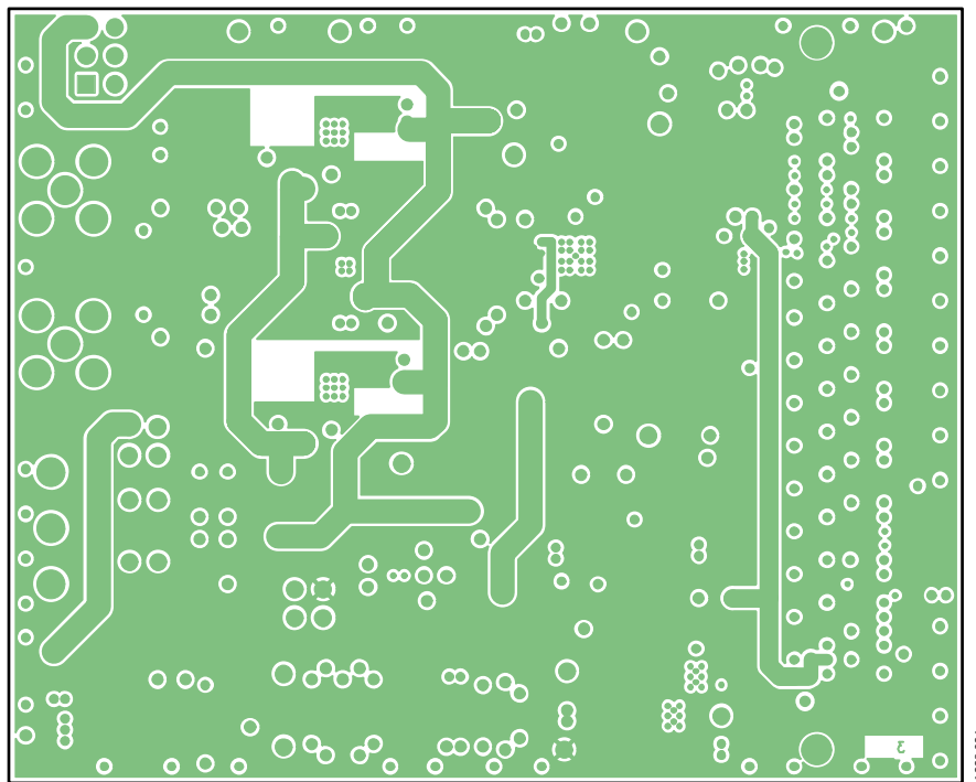
Figure 34. EVAL-AD7960FMCZ Evaluation Board Layer 3—Power
