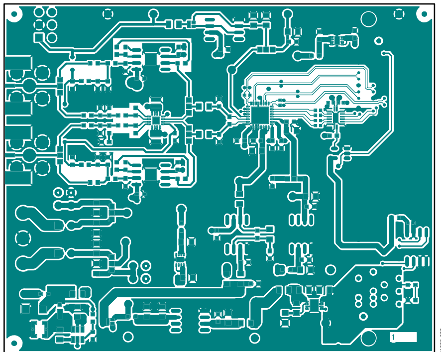
Figure 32. EVAL-AD7960FMCZ Evaluation Board—Top Layer
