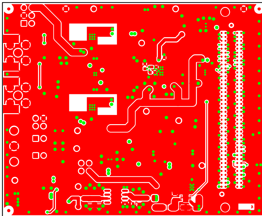
Figure 35. EVAL-AD7960FMCZ Evaluation Board Bottom Layer
