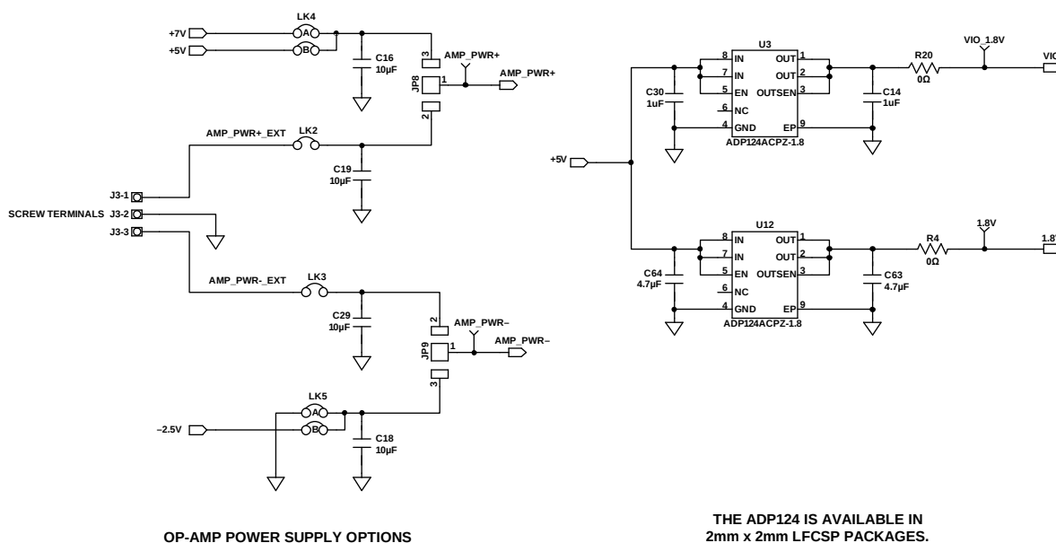
Figure 25. Schematic Page 2
