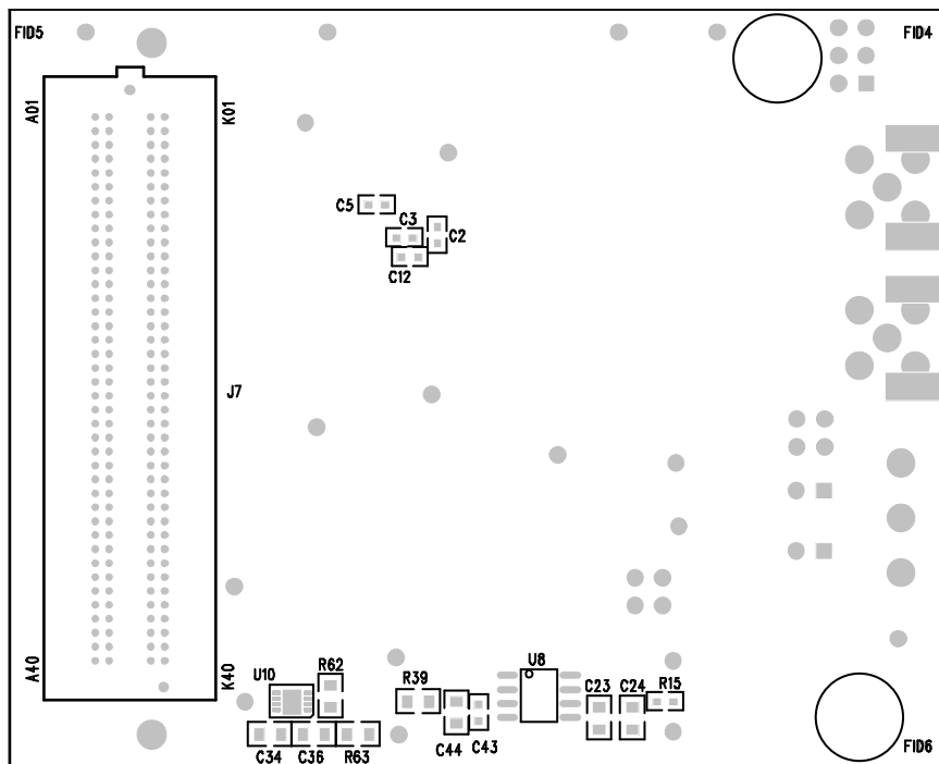
Figure 31. EVAL-AD7960FMCZ Evaluation Board Silkscreen—Bottom Assembly
