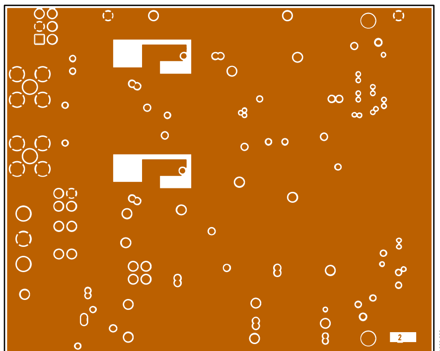
Figure 33. EVAL-AD7960FMCZ Evaluation Board Layer 2—Ground
