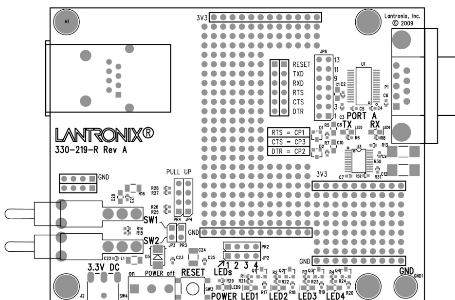
Figure 2-2. XPort Demo Board Layout
