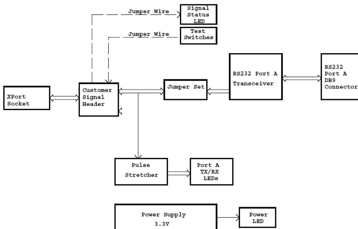
Figure 2-1. Demo Board Block Diagram
